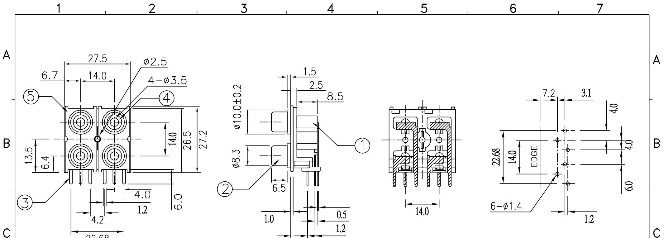
PCB LAYOUT (BOTTOM VIEW)
