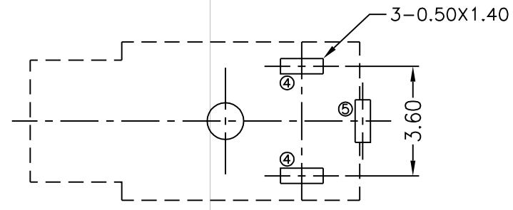
PCB LAYOUT (BOTTOM VIEW)
