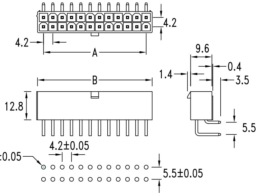
P. C. B . hole dimensions
